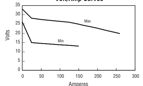
Volt/Amp Curves
